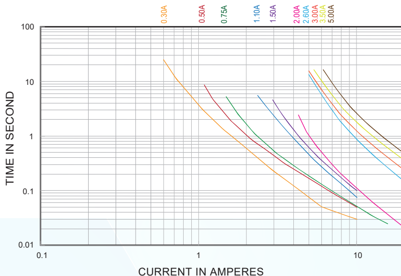
Average Time-Current Curve
